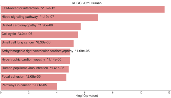
Figure 5. Bar chart of top enriched terms from the KEGG_2021_Human gene set library. The top 10 enriched terms for the input up gene set are displayed based on the -log10(p-value), with the actual p-value shown next to each term. The term at the top has the most significant overlap with the input up gene set in the case of Healthy Control vs Cholangiocarcinoma
