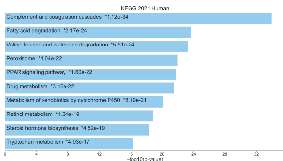
Figure 6. Bar chart of top enriched terms from the KEGG_2021_Human gene set library. The top 10 enriched terms for the input down gene set are displayed based on the -\log_{10}(\text{p-value}) , with the actual p-value shown next to each term. The term at the top has the most significant overlap with the input down gene set in the case of Healthy Control vs Cholangiocarcinoma
