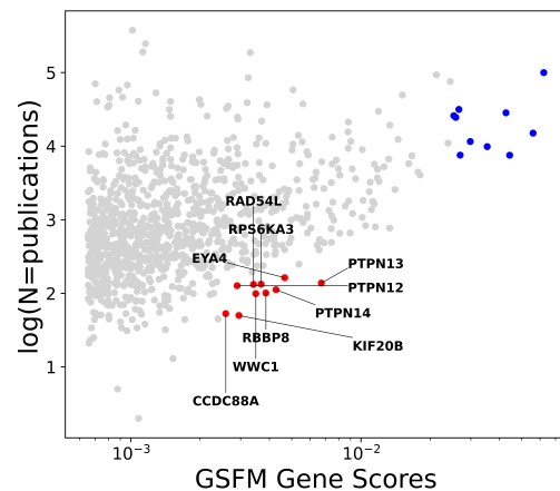
Figure 2. Scatterplot of publication counts vs GSFM gene scores for each of the predicted Cholangiocarcinoma genes. Red points are top 10 understudied genes with high GSFM scores but fewer publications, blue points are top 10 genes with high GSFM scores.
